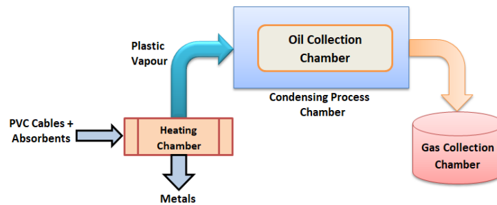
Figure.2 Block Diagram:
