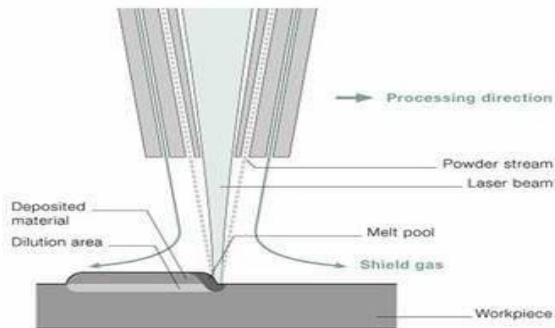
Figure 8. Direct Energy Deposition with metal powder and laser melting
