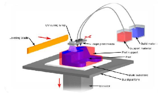
Figure 3. Material Jetting schematics
